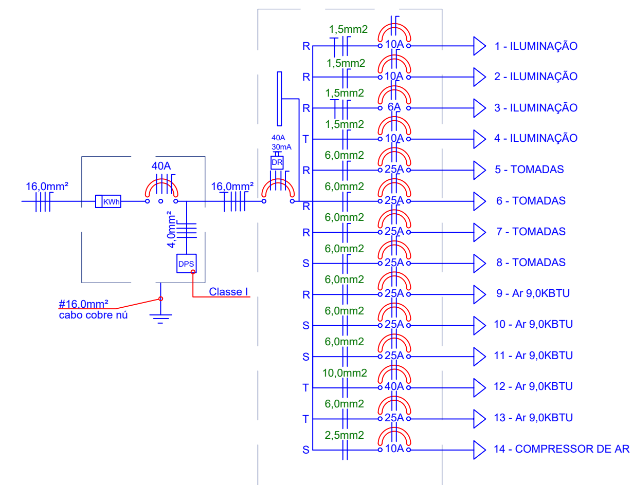
2 DIAGRAMA UNIFILAR S/E
